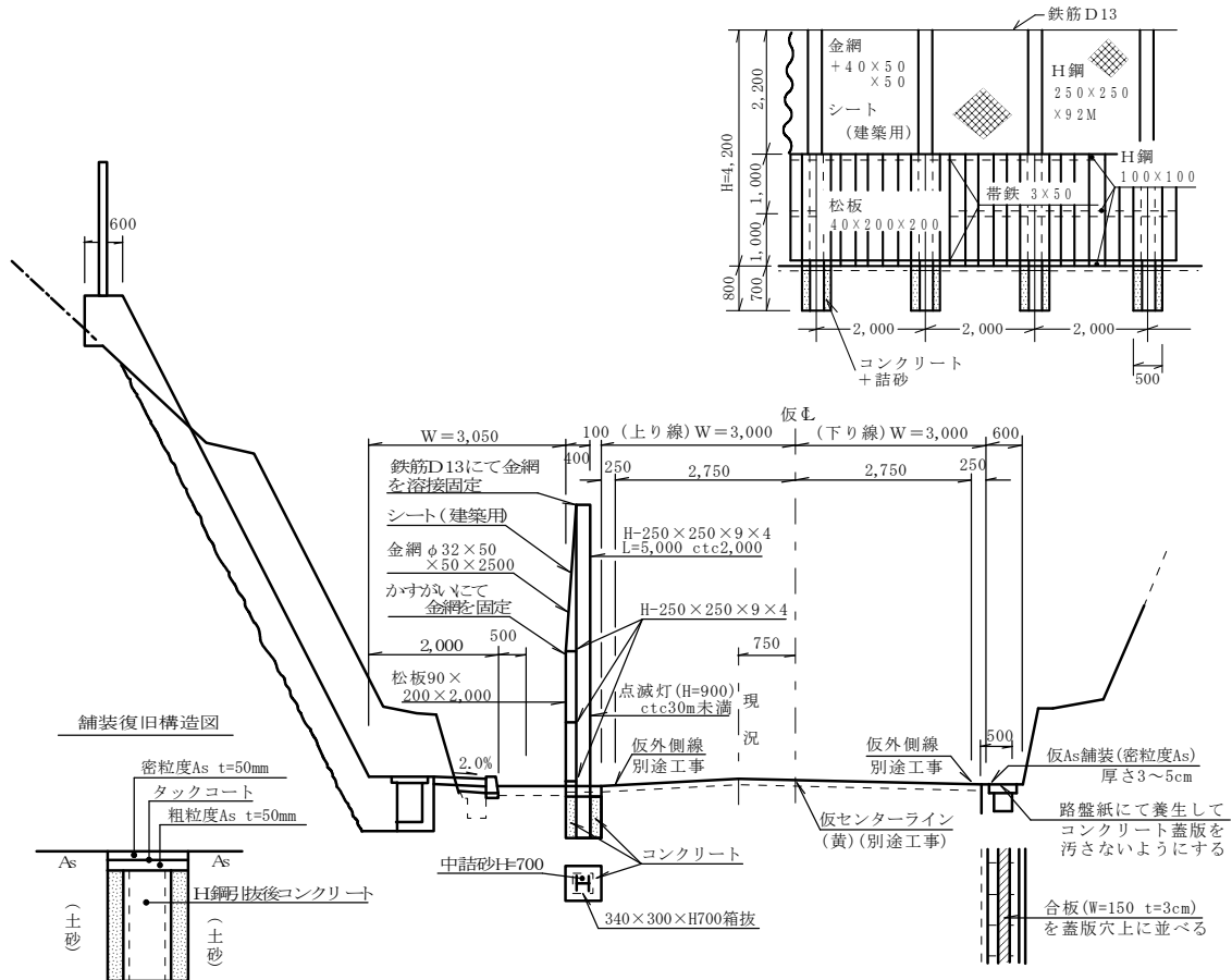
図-6 仮設防護
